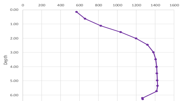
Fig. 2: Conductivity profile by multiparametric probe ( \mu\text{S}/\text{cm} ) in shallow groundwater, BH19.
